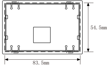
钣金安装开孔尺寸: 83.5mm*54.5mm
